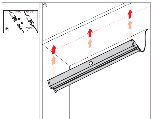
PROFILE LM 10.01.40.XY
